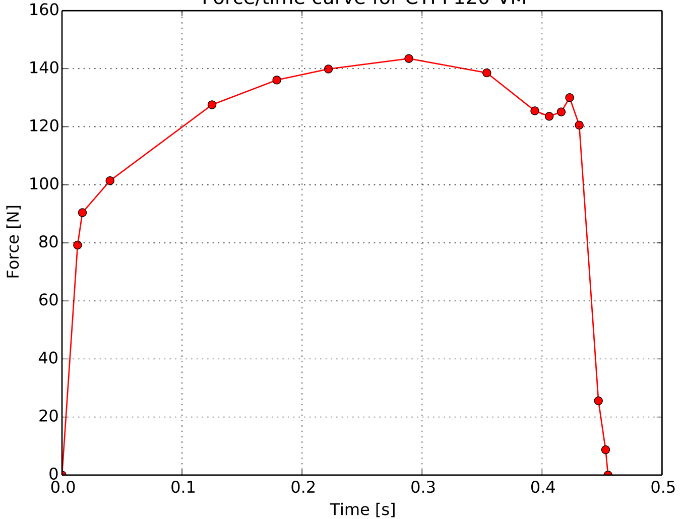
Force/time curve for CTI F120-VM
